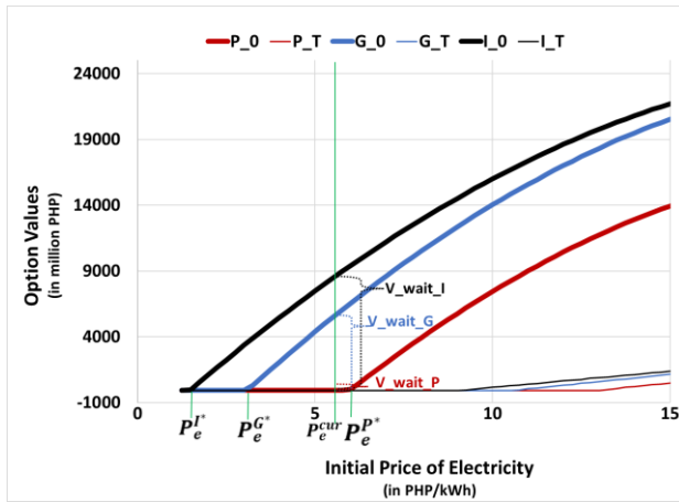
Figure 1. Option value of various WtE investments at different initial prices of electricity. Note: P_0 indicates the option value curve for pyrolysis at initial decision-making period; P_T for terminal period; G_0 for gasification at initial decision-making period; G_T for terminal period; I_0 for incineration at initial decision-making period; I_T for terminal period. V_{wait_I} indicates the value of waiting to invest in incineration; V_{wait_G} for gasification; and V_{wait_P} for pyrolysis. The current price of electricity P_e^{cur} is PHP 5.5508/kWh (May 2018). The optimal timing of investments are P_e^{I*} for incineration; P_e^{G*} for gasification; and P_e^{P*} for pyrolysis.
