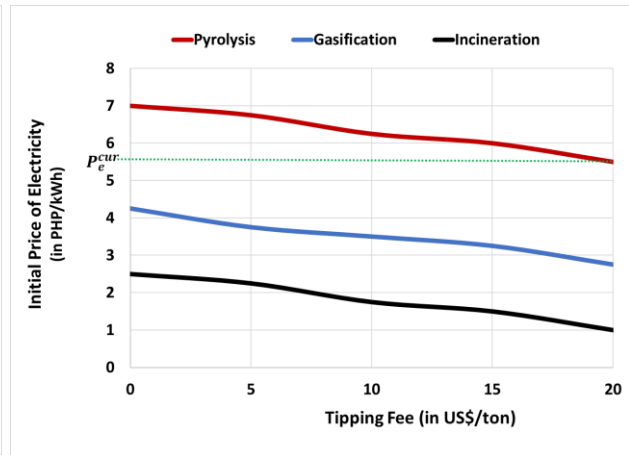
Figure 2. Optimal prices of electricity for investing in WtE technologies at different values of tipping fee.
